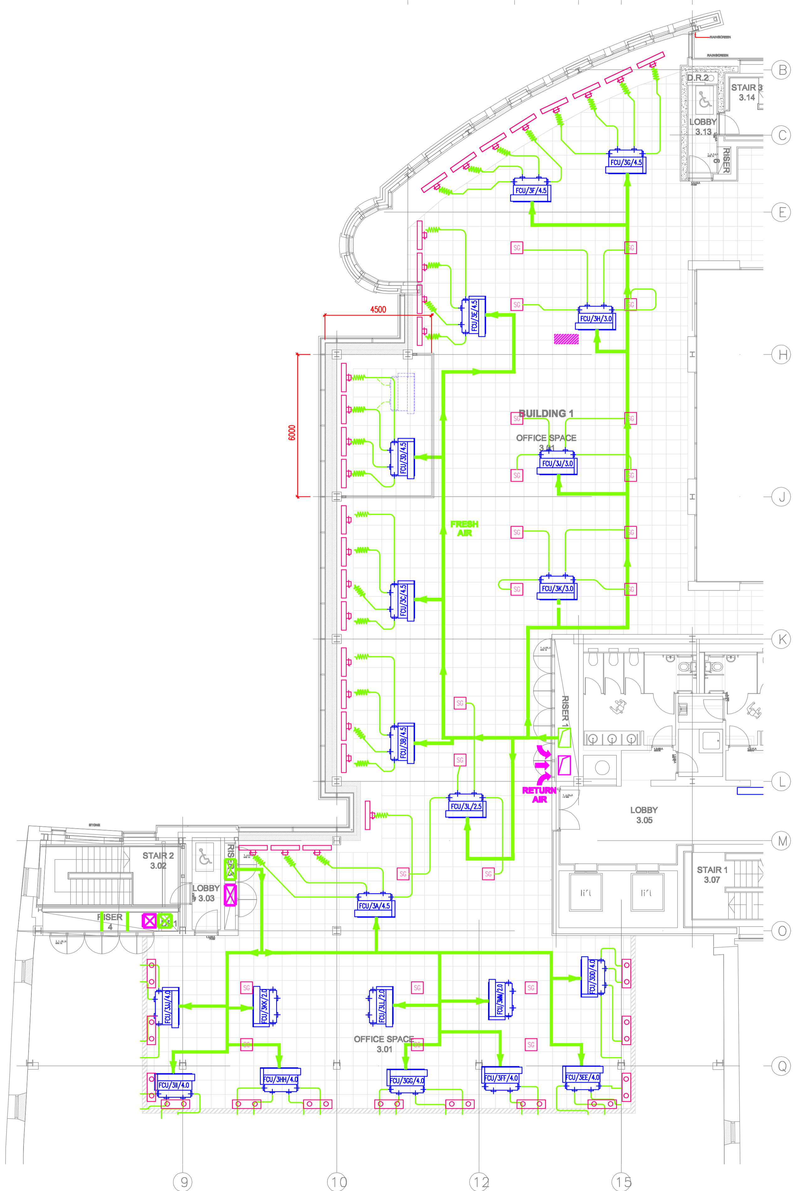
3 Typical Office Air Movement (Scale 1:100) Sketch RYB/07/03/21/C
